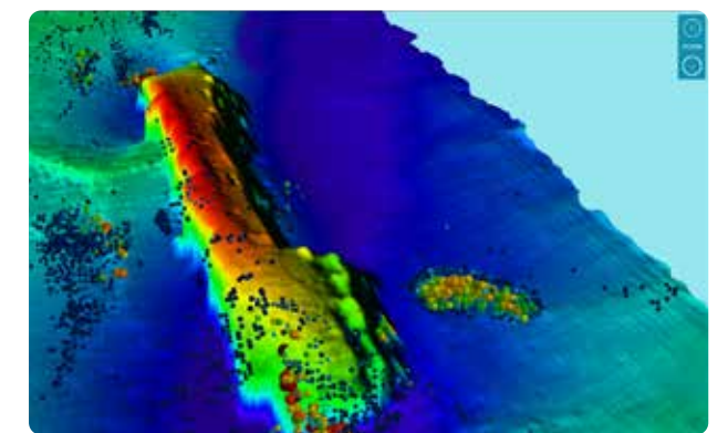
3D map of unknown wreck with water column target Licence showing schools of fish
